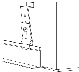
Figure 2 - T-BAR BRACKET DETAIL
